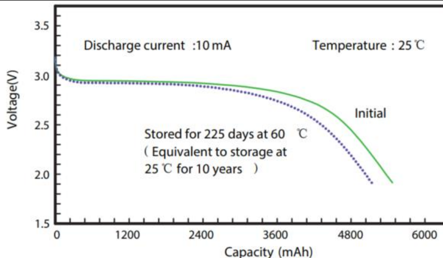
Discharge characteristic
