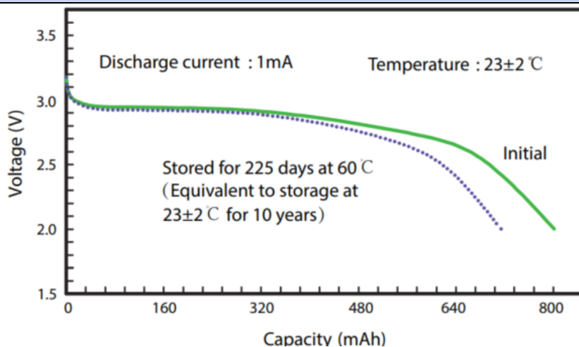
Discharge characteristic
