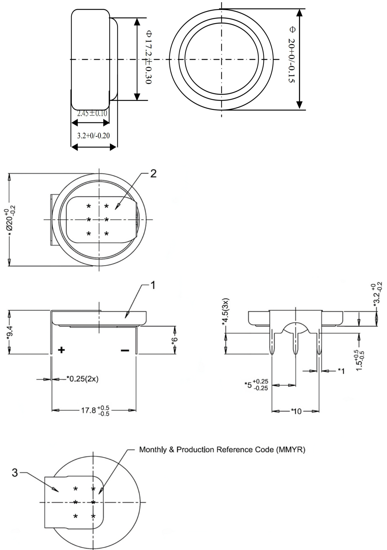
Fig1. Structure of CR2032
