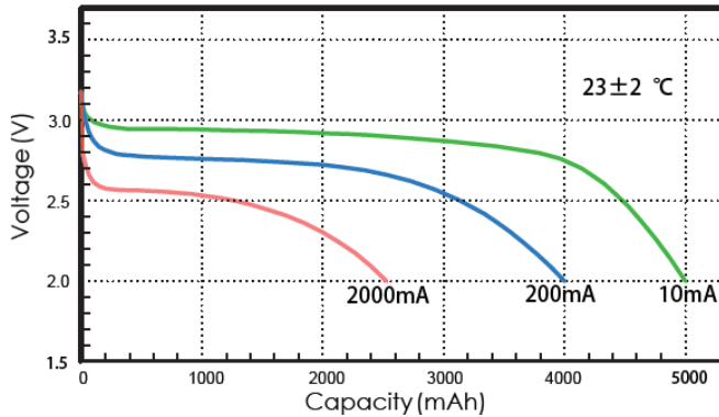
Discharge characteristic
