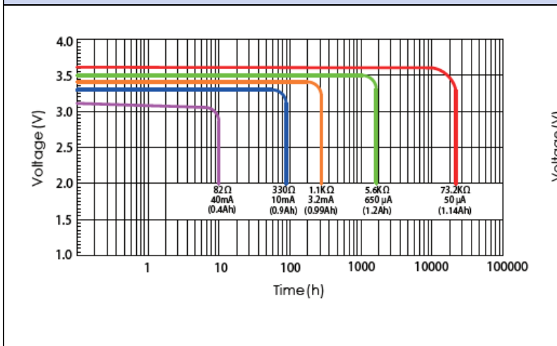
Discharge characteristic
