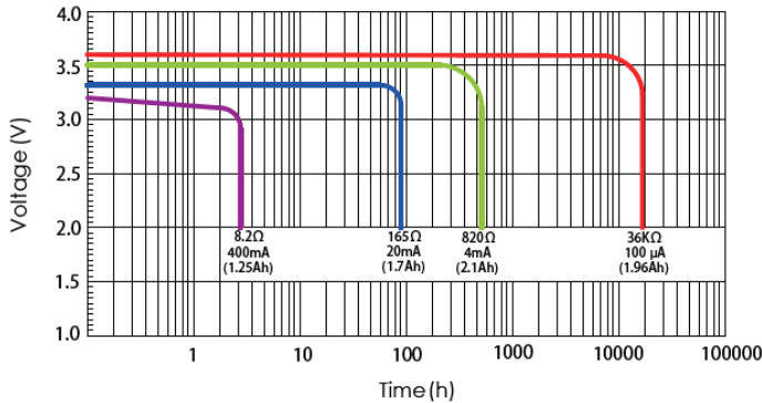
Discharge characteristic
