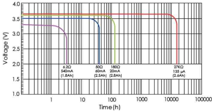
Discharge characteristic
