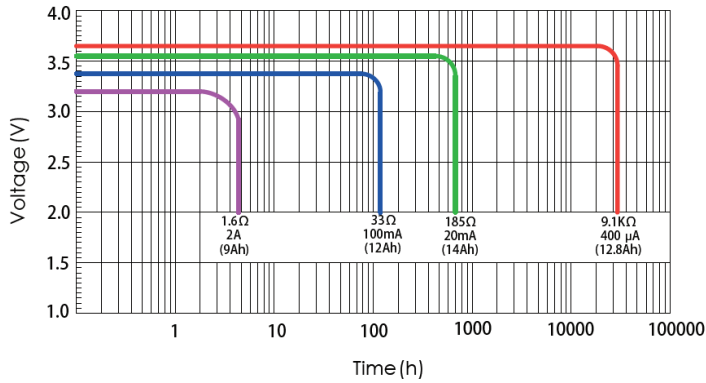
Discharge characteristic
