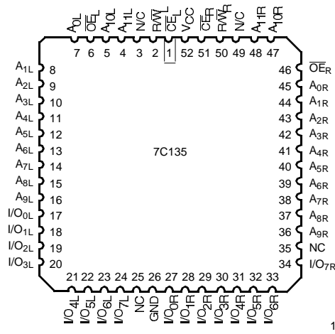
PLCC Top View
