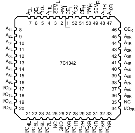
PLCC Top View
