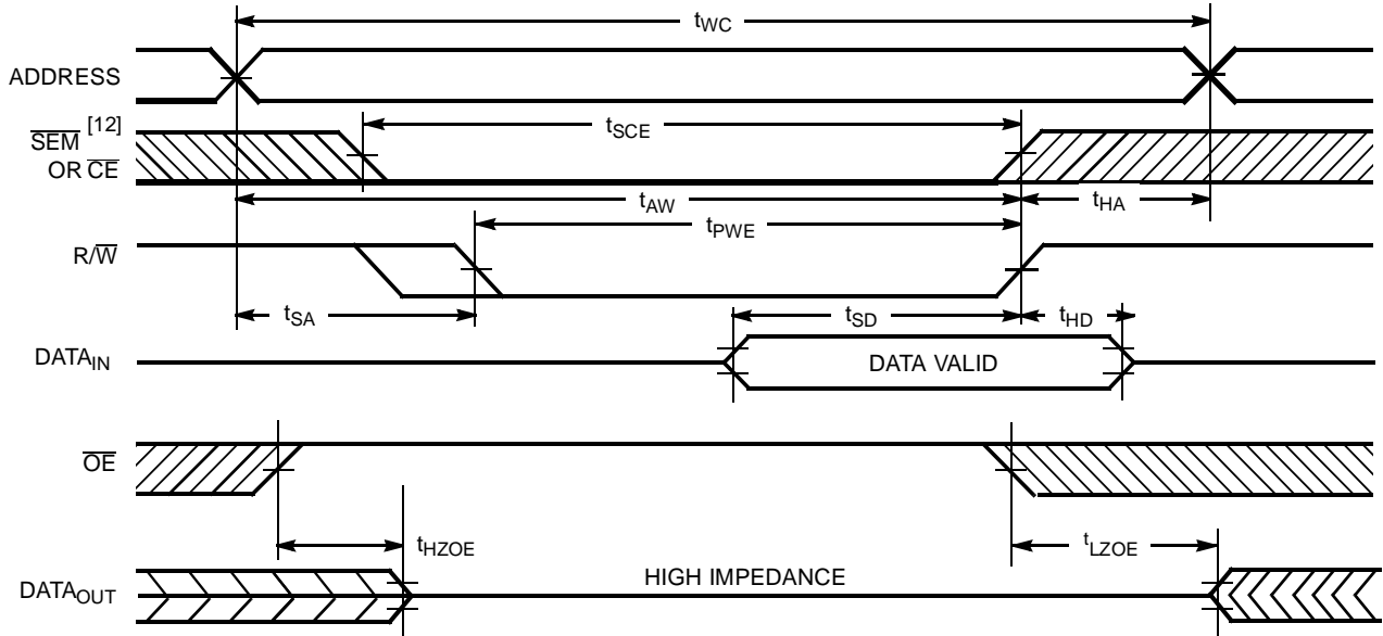
Write Cycle No. 2: R/W Three-States Data I/Os (Either Port) [18, 20]
