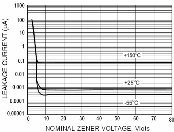
Fig.7 TYPICAL LEAKGE CURRENT
