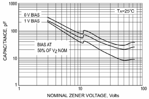
Fig.4 TYPICAL CAPACITANCE
