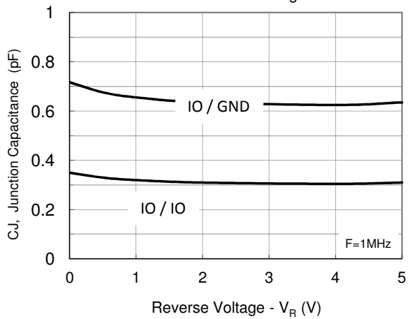
FIG.3 - Junction Capacitance vs. Reverse Voltage
