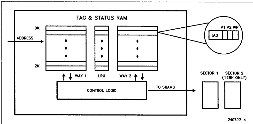
Figure 1.1. 82485 Cache Controller
