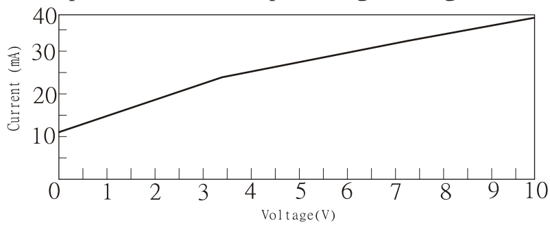
Source Output Current VS Operating Voltage
