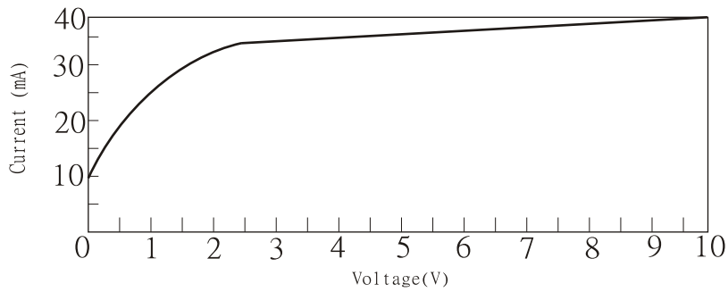
Sink Output Current VS Operating Voltage
