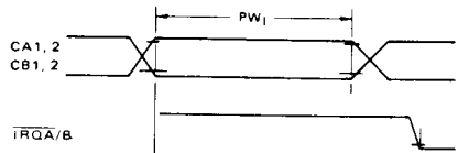
FIGURE 13 — INTERRUPT PULSE WIDTH AND IRQ RESPONSE
