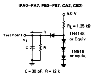
FIGURE 3 — TTL EQUIVALENT TEST LOAD
