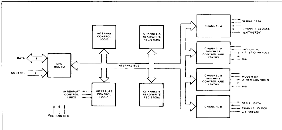
Figure 3 : Block Diagram.
