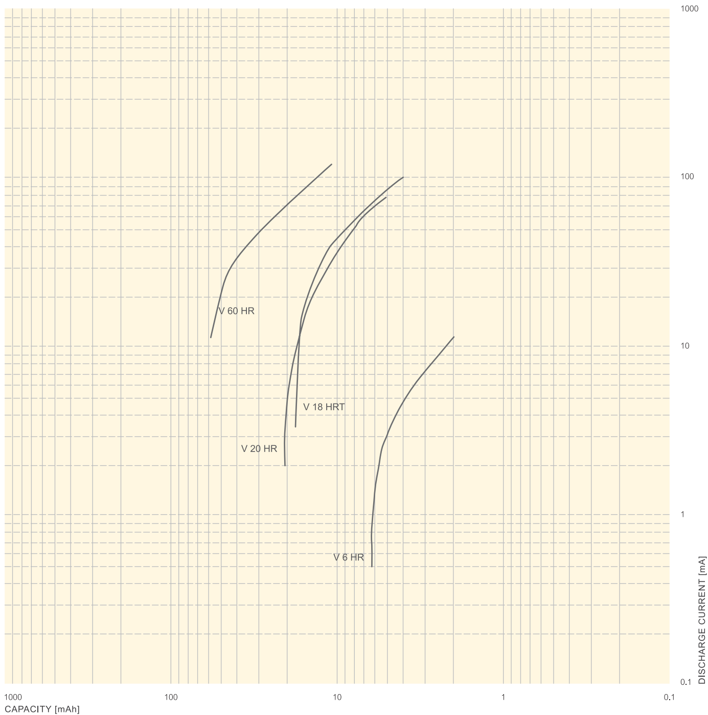
FIG. 38 Discharge characteristics V 60 HR, V 20 HR, V 18 HRT, V 6 HR
