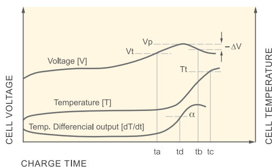
FIG. 26 Charging characteristics (Charging current > 0.5 CA)
