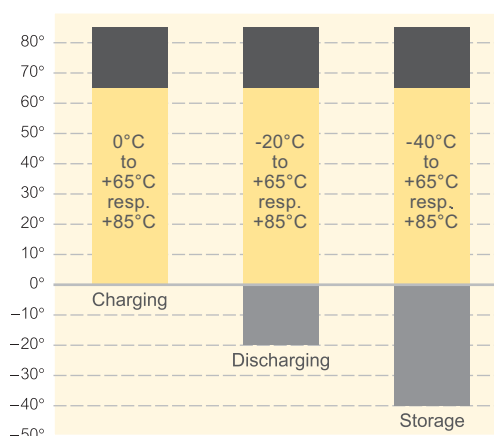
FIG. 39 Permissible temperature range for Ni-MH High Rate Button Cells (+65°C resp. +85°C, depending on type. See also p. 27)
