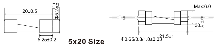
5x20 Size
